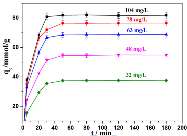
Fig. 10. Effects of reaction time on adsorption capacity: Cr(III) ions concentration (32, 48, 63, 78 and 104 mg/L); adsorbent dosage 0.2 g/L; temperature 25 °C; pH 6.0; and speed agitation 120 rpm.
