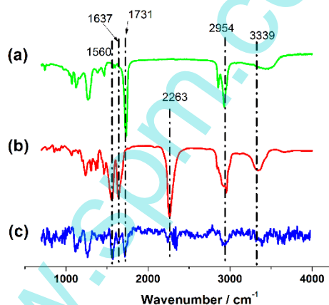
Fig. 1 FT-IR spectra of AVC (a), polyurethane (b), and self-healing products in the crevice (c), respectively.
