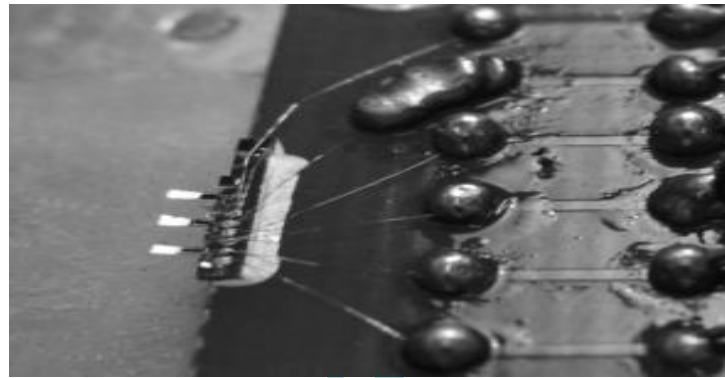
Fig. 2. Picture of PZT microcantilevers on PCB.
