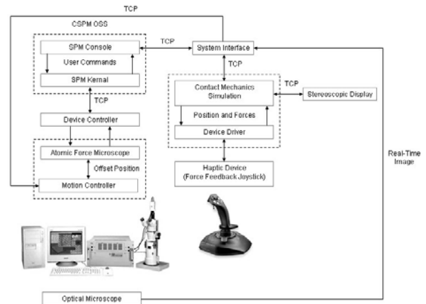
Fig. 2. System architecture of the manipulation system
