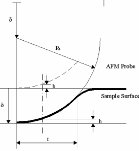
Fig. 4. Contact between two elastic spheres
